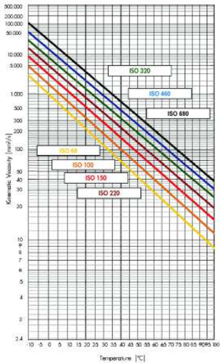
Viscosity - Temperature - Diagram
