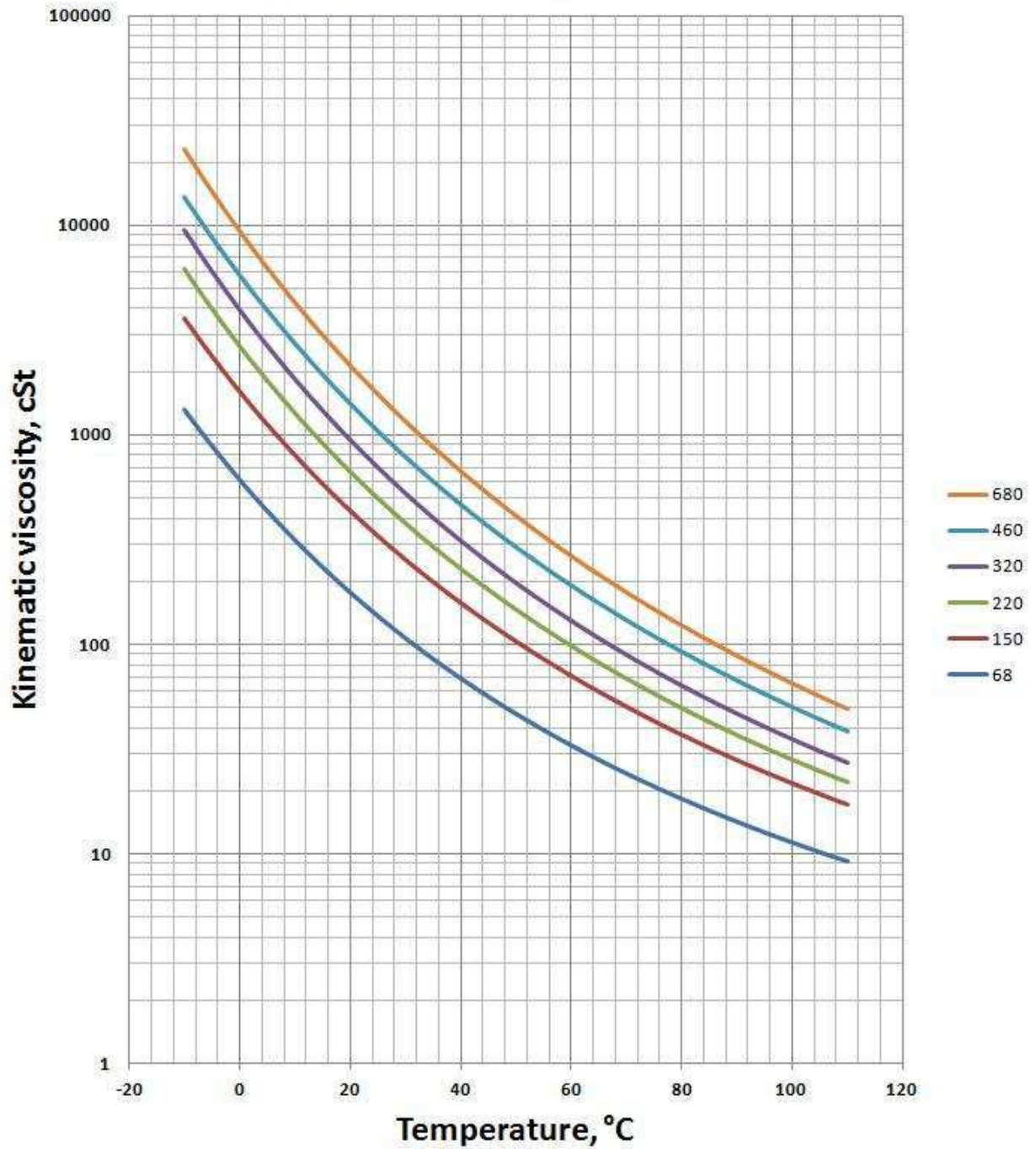
Viscosity - Temperature Diagram for Omala S4 GX
